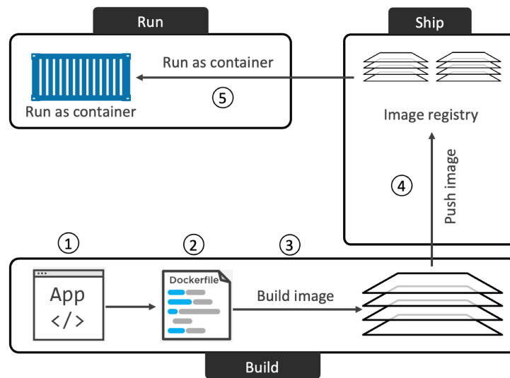
Figure 8.1 - Basic flow of containerizing an app.
