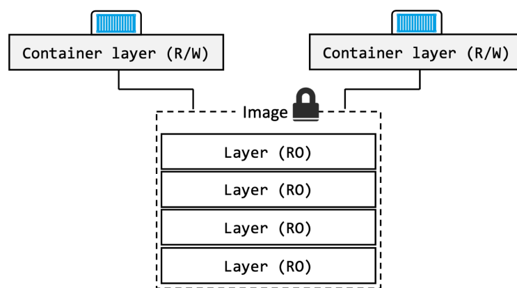
Figure 13.1 Ephemeral container storage.
