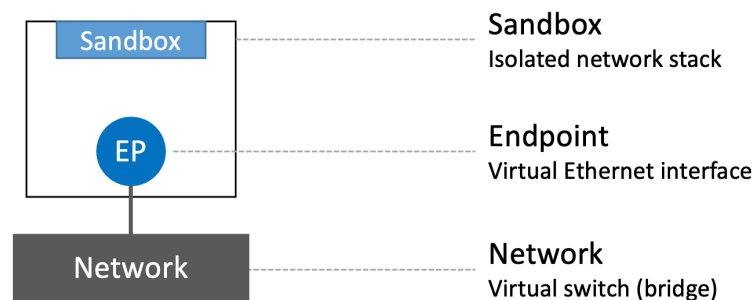
Figure 11.2 The Container Network Model (CNM).
