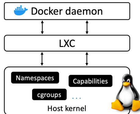
Figure 5.2 Old Docker architecture.
