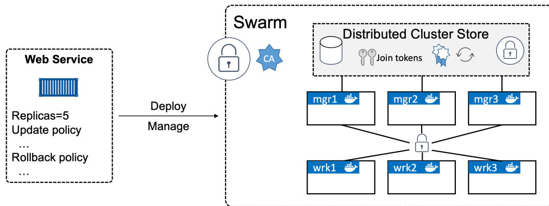
Figure 10.1 High-level swarm.
